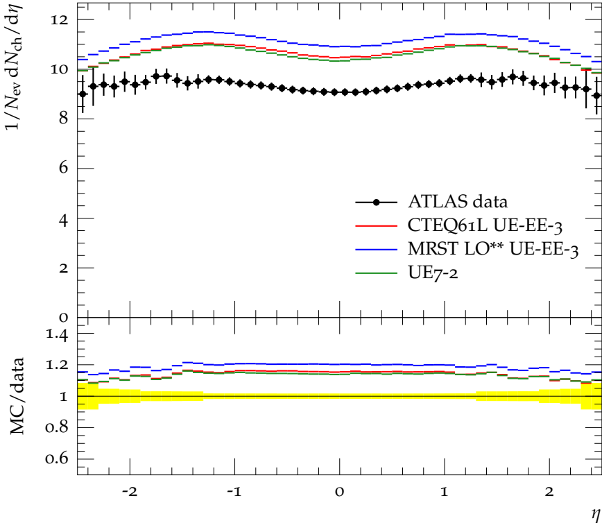
Charged particle \eta at 7 TeV, track p_{\perp} > 100 MeV, for N_{\text{ch}} \geq 20
