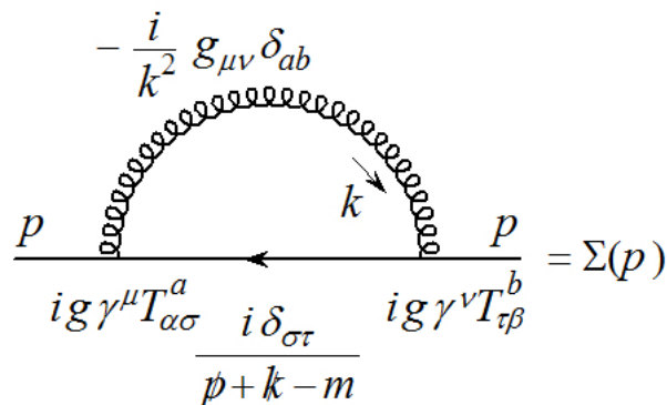
Figure 1: Feynman diagram corresponding to the quark self-energy.
