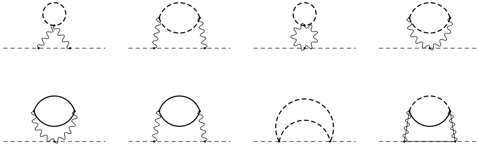
Figure 6.4: MSSM scalar squared masses in gauge-mediated supersymmetry breaking models arise in leading order from these two-loop Feynman graphs. The heavy dashed lines are messenger scalars, the solid lines are messenger fermions, the wavy lines are ordinary Standard Model gauge bosons, and the solid lines with wavy lines superimposed are the MSSM gauginos.
