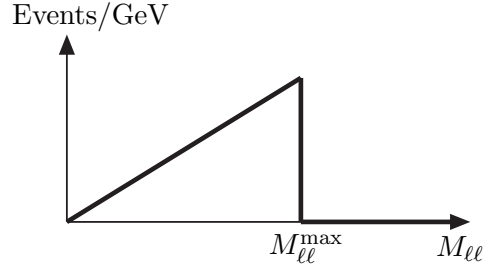
Figure 9.5: The theoretical shape of the dilepton invariant mass distribution from events with \tilde{N}_2 \rightarrow \ell\tilde{\ell} \rightarrow \ell^+\ell^-\tilde{N}_1 . No cuts or detector effects are included. The endpoint is at M_{\ell\ell}^{\max} = m_{\tilde{N}_2}(1 - m_{\tilde{\ell}}^2/m_{\tilde{N}_2}^2)^{1/2}(1 - m_{\tilde{N}_1}^2/m_{\tilde{\ell}}^2)^{1/2} .
