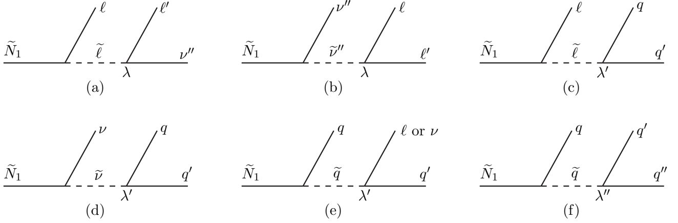
Figure 10.1: Decays of the \tilde{N}_1 LSP in models with R -parity violation, with lepton number not conserved (a)-(e) [see eq. (5.7)], and baryon number not conserved (f) [see eq. (5.8)].
