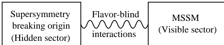
Figure 6.1: The presumed schematic structure for supersymmetry breaking.
