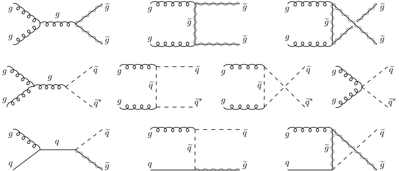
Figure 9.2: Feynman diagrams for gluino and squark production at hadron colliders from gluon-gluon and gluon-quark fusion.
