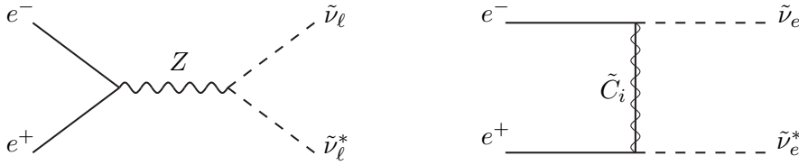
Figure 9.9: Diagrams for sneutrino pair production at e^+e^- colliders.
