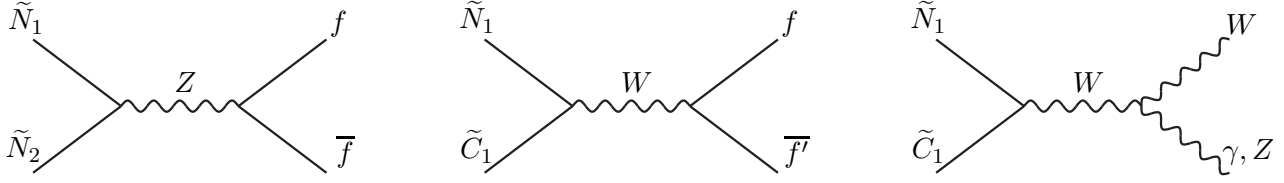
Figure 9.14: Some contributions to the co-annihilation of dark matter \tilde{N}_1 LSPs with slightly heavier \tilde{N}_2 and \tilde{C}_1 . All three diagrams are particularly important if the LSP is higgsino-like, and the last two diagrams are important if the LSP is wino-like.
