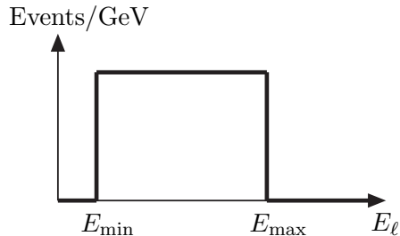
Figure 9.12: The theoretical shape of the lepton energy distribution from events with e^+e^- \rightarrow \tilde{\ell}^+\tilde{\ell}^- \rightarrow \ell^+\ell^-\tilde{N}_1\tilde{N}_1 at a future linear collider. No cuts or initial state radiation or beamstrahlung or detector effects are included. The endpoints are E_{\max,\min} = \frac{\sqrt{s}}{4}(1 - m_{\tilde{N}_1}^2/m_{\tilde{\ell}}^2)[1 \pm (1 - 4m_{\tilde{\ell}}^2/s)^{1/2}] , allowing precision reconstruction of both \tilde{\ell} and \tilde{N}_1 masses.
