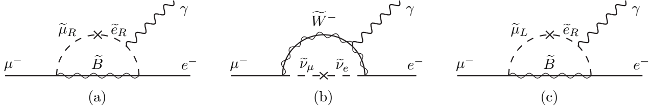
Figure 5.6: Some of the diagrams that contribute to the process \mu^- \rightarrow e^- \gamma in models with lepton flavor-violating soft supersymmetry breaking parameters (indicated by \times ). Diagrams (a), (b), and (c) contribute to constraints on the off-diagonal elements of \mathbf{m}_{\tilde{\mathbf{e}}}^2 , \mathbf{m}_{\tilde{\mathbf{L}}}^2 , and \mathbf{a}_{\mathbf{e}} , respectively.
