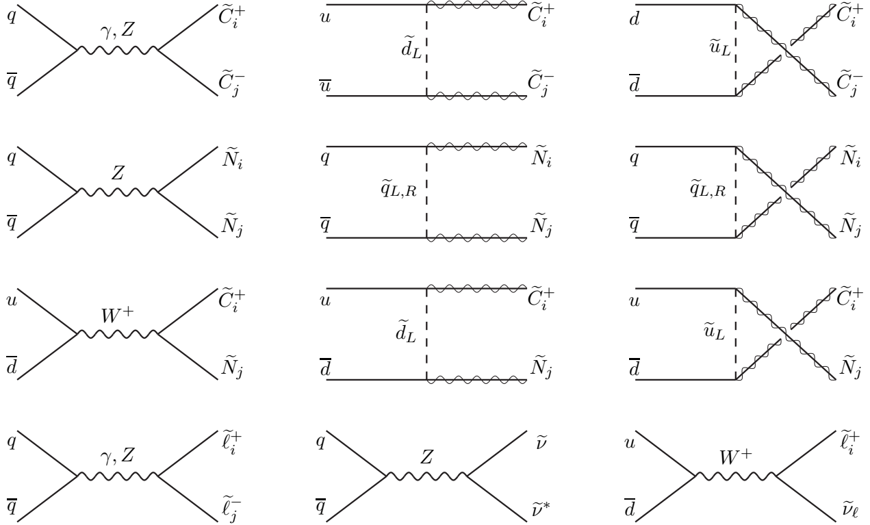
Figure 9.1: Feynman diagrams for electroweak production of sparticles at hadron colliders from quark-antiquark annihilation. The charginos and neutralinos in the t -channel diagrams only couple because of their gaugino content, for massless initial-state quarks, and so are drawn as wavy lines superimposed on solid.
