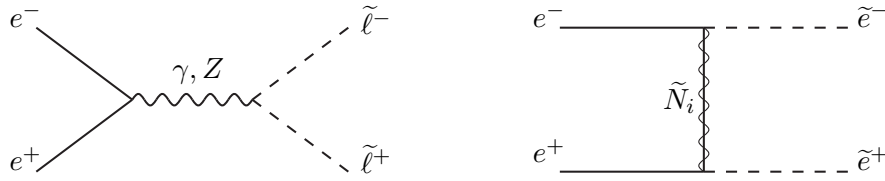
Figure 9.8: Diagrams for charged slepton pair production at e^+e^- colliders.
