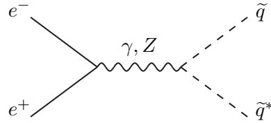
Figure 9.10: Diagram for squark production at e^+e^- colliders.
