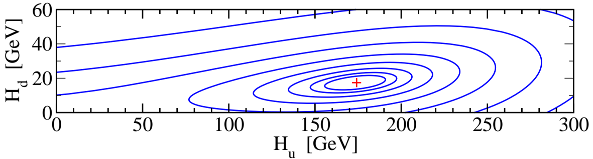
Figure 7.1: A contour map of the Higgs potential, for a typical case with \tan\beta \approx -\cot\alpha \approx 10 . The minimum of the potential is marked by +, and the contours are equally spaced equipotentials. Oscillations along the shallow direction, with H_u^0/H_d^0 \approx 10 , correspond to the mass eigenstate h^0 , while the orthogonal steeper direction corresponds to the mass eigenstate H^0 .
