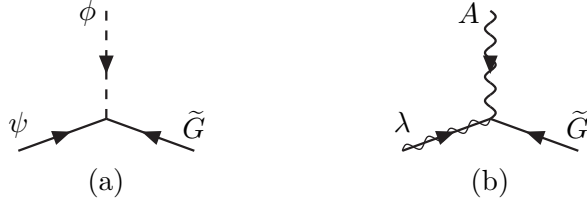
Figure 6.2: Goldstino/gravitino \tilde{G} interactions with superpartner pairs (\phi, \psi) and (\lambda, A) .
