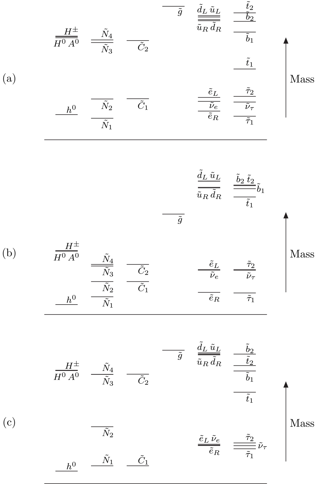
Figure 7.5: Three sample schematic mass spectra for the undiscovered particles in the MSSM, for (a) minimal supergravity with m_0^2 \ll m_{1/2}^2 , (b) minimal GMSB with N_5 = 1 , and (c) AMSB with an extra m_0^2 for scalars. These spectra are presented for entertainment purposes only! No warranty, expressed or implied, guarantees that they look anything like the real world.
