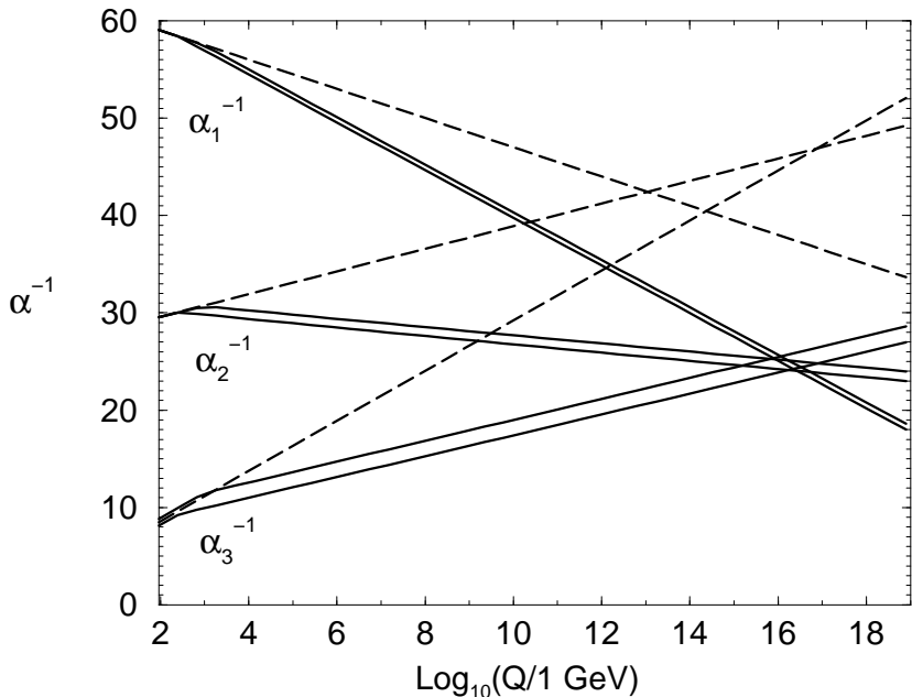
Figure 5.8: RG evolution of the inverse gauge couplings \alpha_a^{-1}(Q) in the Standard Model (dashed lines) and the MSSM (solid lines). In the MSSM case, the sparticle mass thresholds are varied between 250 GeV and 1 TeV, and \alpha_3(m_Z) between 0.113 and 0.123. Two-loop effects are included.
