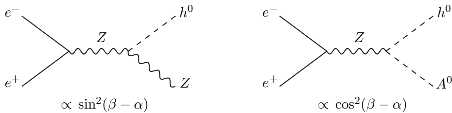
Figure 9.11: Diagrams for neutral Higgs scalar boson production at e^+e^- colliders.
