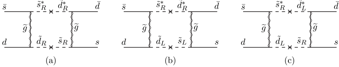
Figure 5.7: Some of the diagrams that contribute to K^0 \leftrightarrow \bar{K}^0 mixing in models with strangeness-violating soft supersymmetry breaking parameters (indicated by \times ). These diagrams contribute to constraints on the off-diagonal elements of (a) \mathbf{m}_{\tilde{\mathbf{d}}}^2 , (b) the combination of \mathbf{m}_{\tilde{\mathbf{d}}}^2 and \mathbf{m}_{\tilde{\mathbf{Q}}}^2 , and (c) \mathbf{a}_{\mathbf{d}} .
