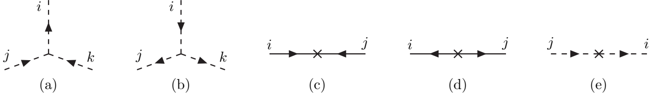
Figure 3.2: Supersymmetric dimensionful couplings: (a) (scalar) 3 interaction vertex M_{in}^* y^{jkn} and (b) the conjugate interaction M^{in} y_{jkn}^* , (c) fermion mass term M^{ij} and (d) conjugate fermion mass term M_{ij}^* , and (e) scalar squared-mass term M_{ik}^* M^{kj} .
