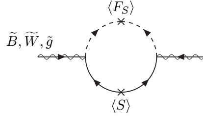
Figure 6.3: Contributions to the MSSM gaugino masses in gauge-mediated supersymmetry breaking models come from one-loop graphs involving virtual messenger particles.
