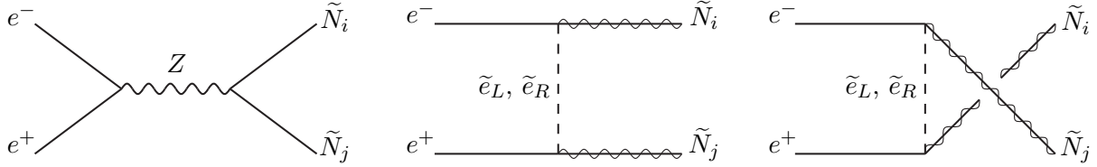
Figure 9.7: Diagrams for neutralino pair production at e^+e^- colliders.
