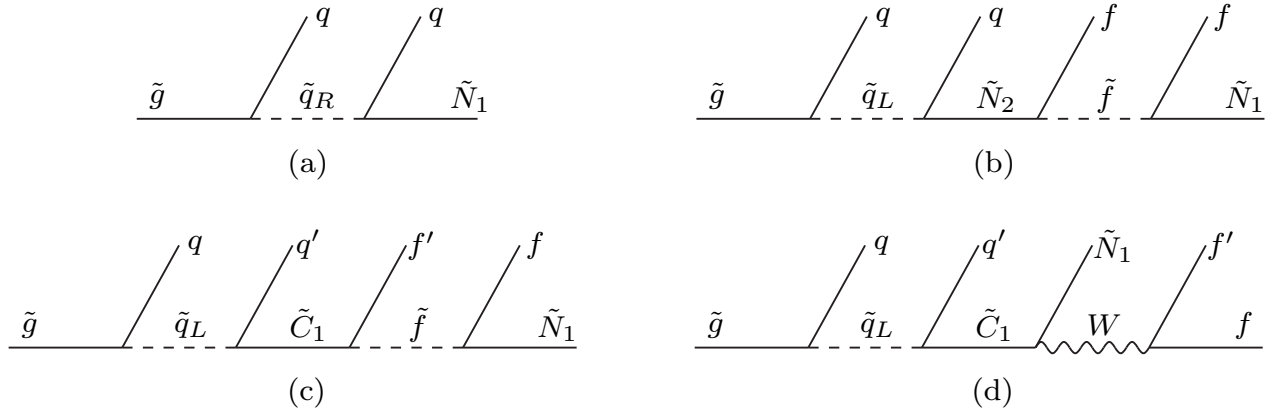
Figure 8.2: Some of the many possible examples of gluino cascade decays ending with a neutralino LSP in the final state. The squarks appearing in these diagrams may be either on-shell or off-shell, depending on the mass spectrum of the theory.
