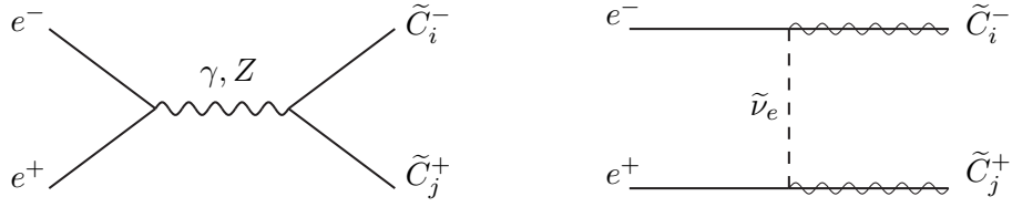
Figure 9.6: Diagrams for chargino pair production at e^+e^- colliders.
