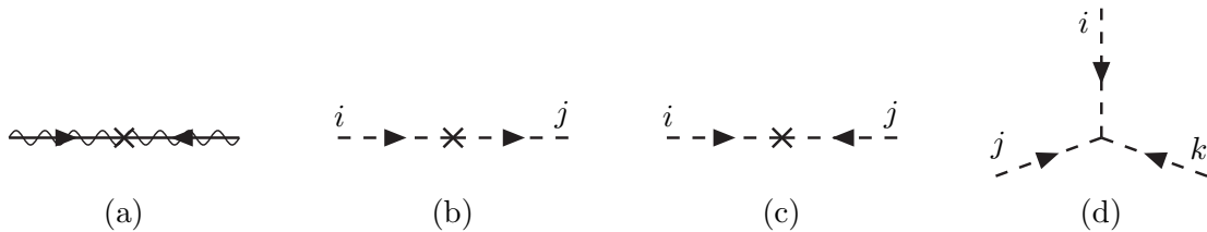
Figure 4.1: Soft supersymmetry-breaking terms: (a) Gaugino mass M_a ; (b) non-analytic scalar squared mass (m^2)_j^i ; (c) analytic scalar squared mass b^{ij} ; and (d) scalar cubic coupling a^{ijk} .
