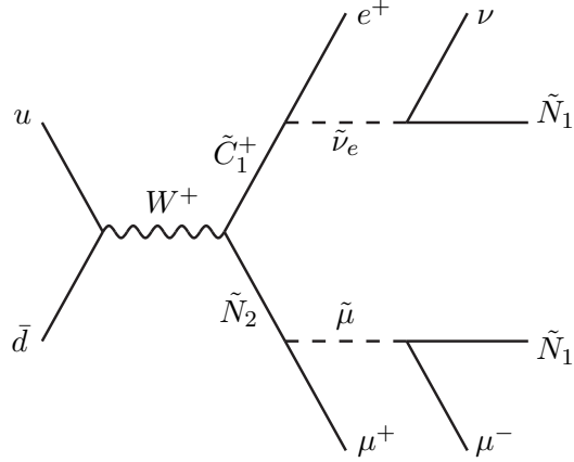
Figure 9.4: A complete Feynman diagram for a clean (no high- p_T hadronic jets) triplepton event at a hadron collider, from production of an on-shell neutralino and a chargino, with subsequent leptonic decays, leading in this case to \mu^+\mu^-e^+ + \cancel{E}_T .
