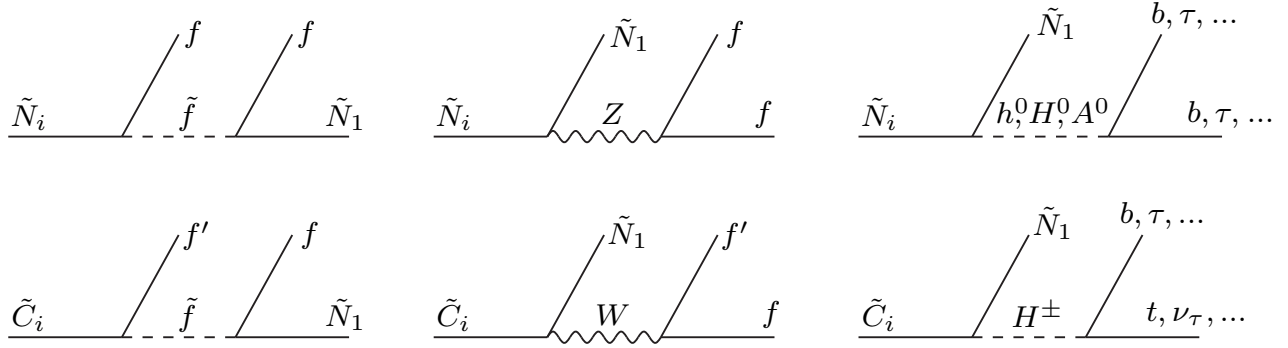
Figure 8.1: Feynman diagrams for neutralino and chargino decays with \tilde{N}_1 in the final state. The intermediate scalar or vector boson in each case can be either on-shell (so that actually there is a sequence of two-body decays) or off-shell, depending on the sparticle mass spectrum.
