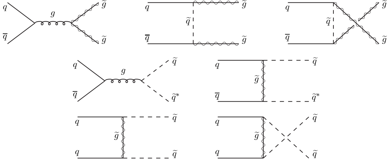
Figure 9.3: Feynman diagrams for gluino and squark production at hadron colliders from strong quark-antiquark annihilation and quark-quark scattering.
