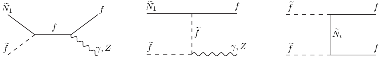
Figure 9.15: Some contributions to the co-annihilation of dark matter \tilde{N}_1 LSPs with slightly heavier sfermions, which in popular models are most plausibly staus (or perhaps top squarks).
