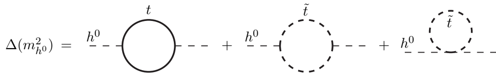
Figure 7.2: Contributions to the MSSM lightest Higgs mass from top-quark and top-squark one-loop diagrams. Incomplete cancellation, due to soft supersymmetry breaking, leads to a large positive correction to m_{h^0}^2 in the limit of heavy top squarks.
