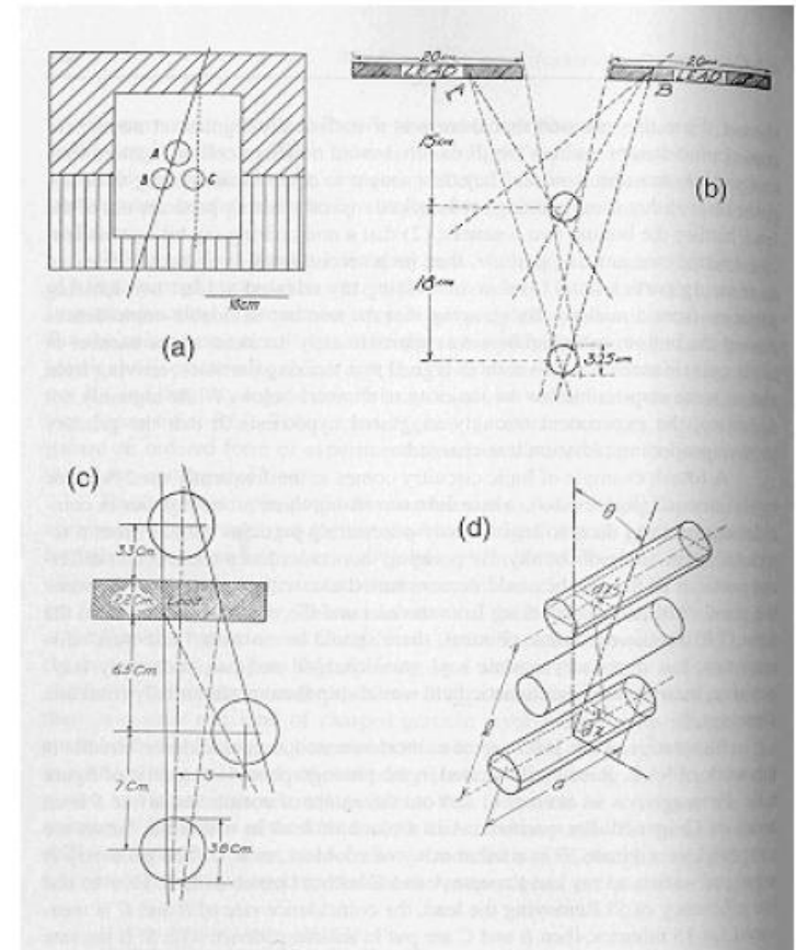
Early coincidence counting experiment
