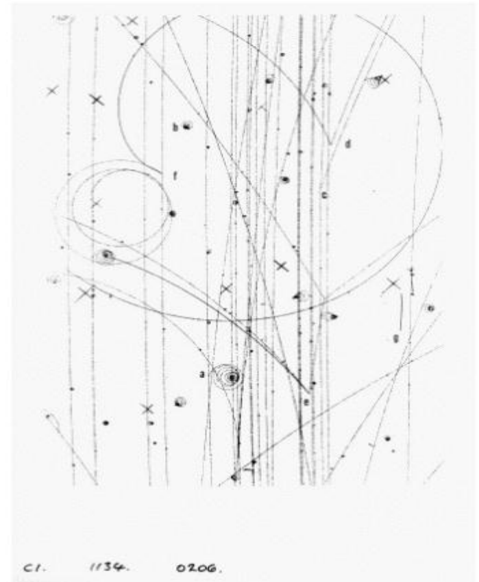
Bubble chamber photograph
