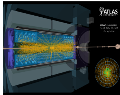
Simulation of t\bar{t} event in ATLAS tracker with 200 pileup collisions
