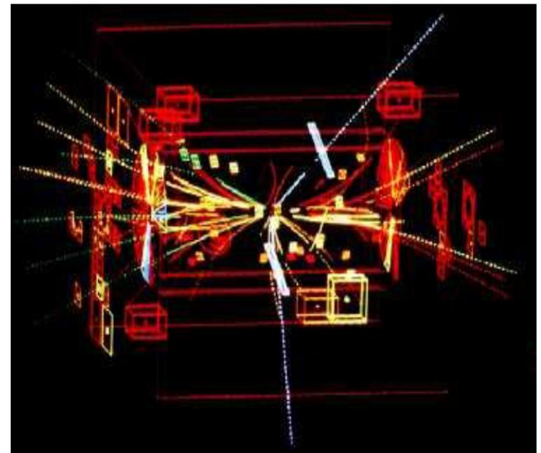
Z-Event at UA1 / CERN
