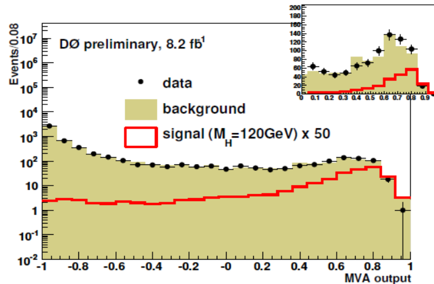
(c) M_H = 120\text{ GeV}
