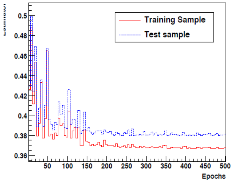
MLP Convergence Test
