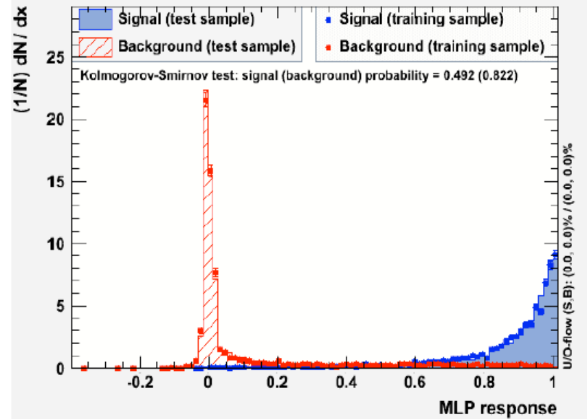
TMVA overtraining check for classifier: MLP
