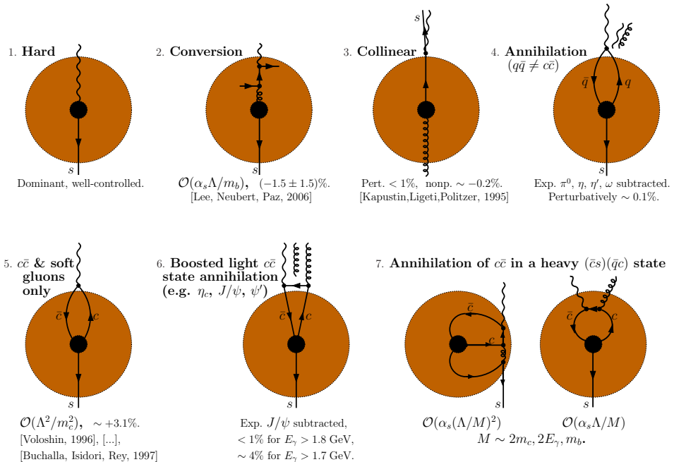
Fig. 1. Energetic photon production ( E_\gamma \gtrsim \frac{m_b}{3} ) in charmless decays of the \bar{B} meson. The first and second rows describe situations without and with long-distance charm loops, respectively (see the text).
