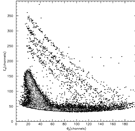
Fig. 2. Energy versus angle plot for one \Delta E - E telescope in the ^{132}\text{Sn}(d, p) experiment.
