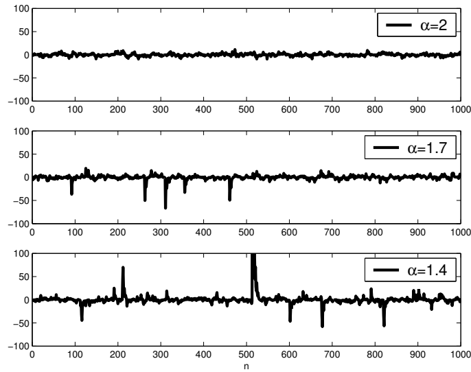
Fig. 1. The realizations of PARMA(1,1) model with SaS innovations for \alpha = 2 (top panel), \alpha = 1.7 (middle panel) and \alpha = 1.4 (bottom panel).
