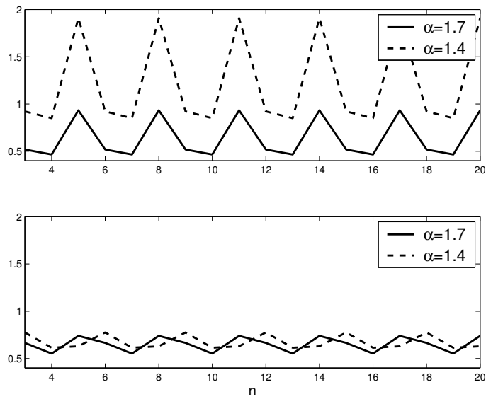
Fig. 2. The codifference CD(X_n, X_{n+k}) (top panel) and the covariation CV(X_n, X_{n+k}) (bottom panel) for PARMA(1,1) model with SaS innovations for \alpha = 1.7 (solid line) and \alpha = 1.4 (dotted line) versus n = 3, 4, \dots, 20 for k = 5 .
