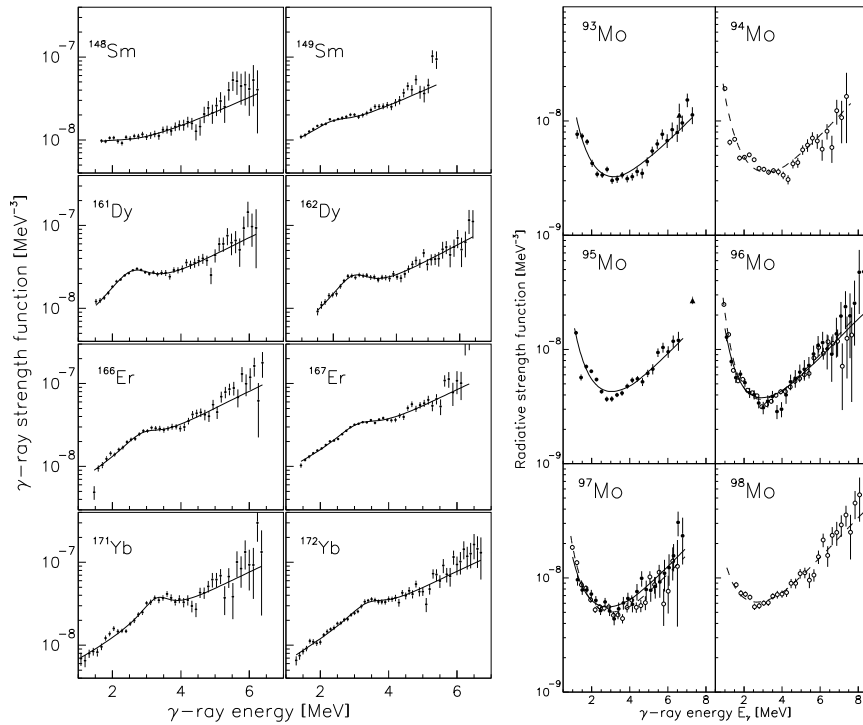
Fig. 1. Normalized RSFs for ^{148,149}\text{Sm} , ^{161,162}\text{Dy} , ^{166,167}\text{Er} , ^{171,172}\text{Yb} (left panel) and ^{93-98}\text{Mo} (right panel). The circles are the experimental data. In the right panel the filled and open circles are data from the (^3\text{He},\alpha) and (^3\text{He},^3\text{He}') reactions, respectively. The solid and dashed lines are fits to the respective reactions.
