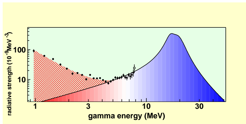
Fig. 2. Data points: The experimental radiative strength function(RSF) for ^{57}\text{Fe} . Open circle: Lowest previous data point from literature. Solid line: A standard nuclear theory prediction (Lorentzian) for the tail of the GEDR. Hatched area: Excess yield of low-energy radiation.
