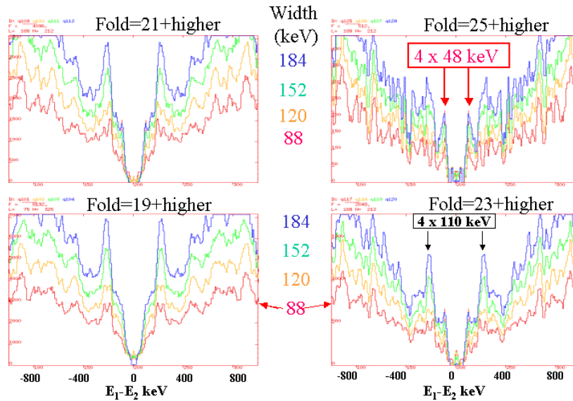
Fig. 3. Perpendicular cuts across rotational planes for ^{126}\text{Xe} with four different thresholds on the coincidence fold and for four widths of the cuts between 88 and 184 keV [20].
