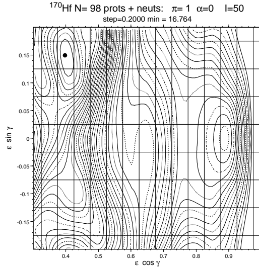
Fig. 1. Potential-energy surface for ^{170}\text{Hf} at spin 50 \hbar for parity and signature (+,0) calculated using the UC code. The energy separation of the contour lines is 200 keV.
