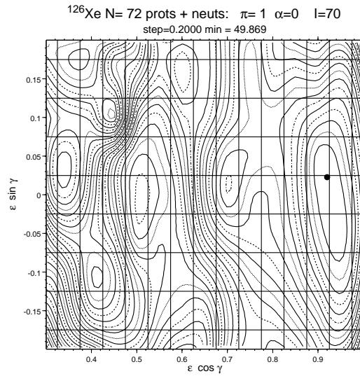
Fig. 2. Potential-energy surface for ^{126}\text{Xe} at spin 70 \hbar for parity and signature (+,0) calculated using the UC code. The energy separation of the contour lines is 200 keV.
