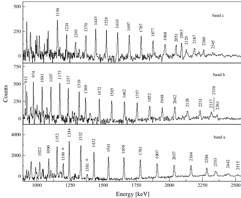
Fig. 5. Gamma-ray coincidence spectra of three new ND bands in ^{126}\text{Xe} . For band a, lower-lying transitions are marked by an asterisk.
