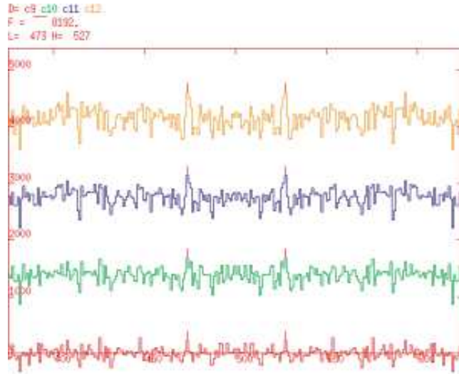
Fig. 7. Differences of perpendicular cuts, 204 keV wide, at 1440 keV across rotational planes with \delta = 12 keV from data measured at 261 and 255 MeV beam energy for ^{126}\text{Ba} . The four spectra, from bottom to top, are for thresholds of 22, 24, 26 and 28 on the coincidence fold [21].
