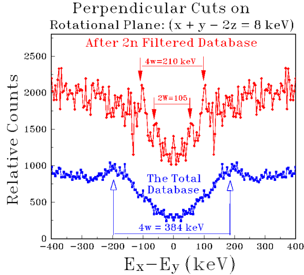
Fig. 6. Perpendicular cuts, 142 keV wide, across the rotational planes at 1440 keV for the ^{126}\text{Ba} filtered data, upper spectrum, and for the total data set, lower spectrum [20, 21].
