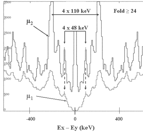
Fig. 4. Result of a fluctuation analysis on a perpendicular cut at 1360 keV across a rotational plane for ^{126}\text{Xe} [31].
