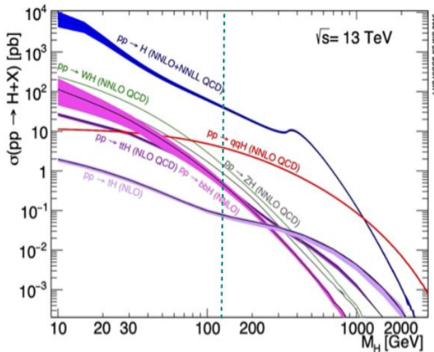
production cross section
