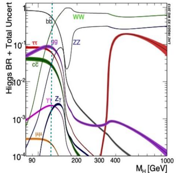
branching ratio
