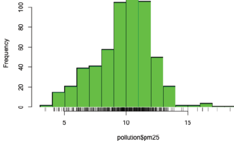
Histogram of pollution$pm25
