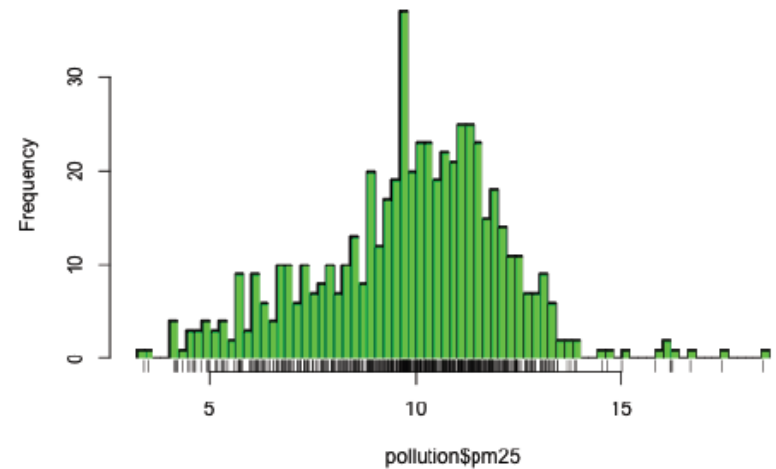
Histogram of pollution$pm25
